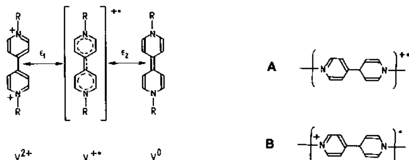
Fig. 17. Reduction states of viologen.
