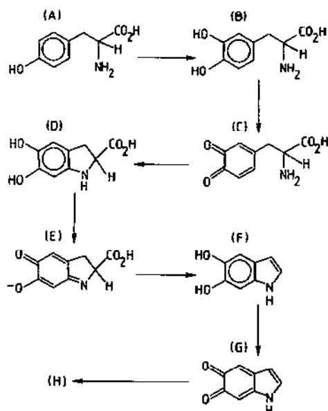
Fig. 6. Enzymatic pathway for the formation of melanin from dopa [174]. (A) tyrosine; (B) dopa; (C) dopaquinone; (D) leucodopachrome; (E) dopachrome; (F) 5,6-dihydroxyindole; (G) indole-5,6-quinone; (H) melanin polymer.
