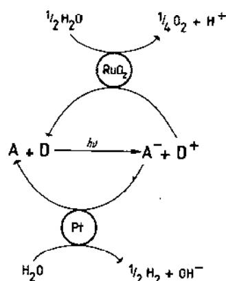
Fig. 22. Schematic representation of a coupled water-splitting system [680].
